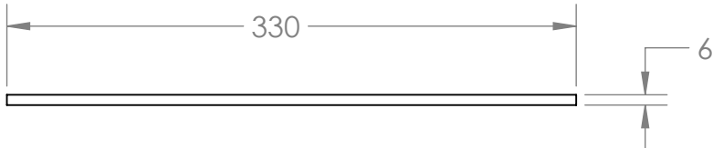
1134 SIDE FRAME
